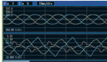
Harmonics
